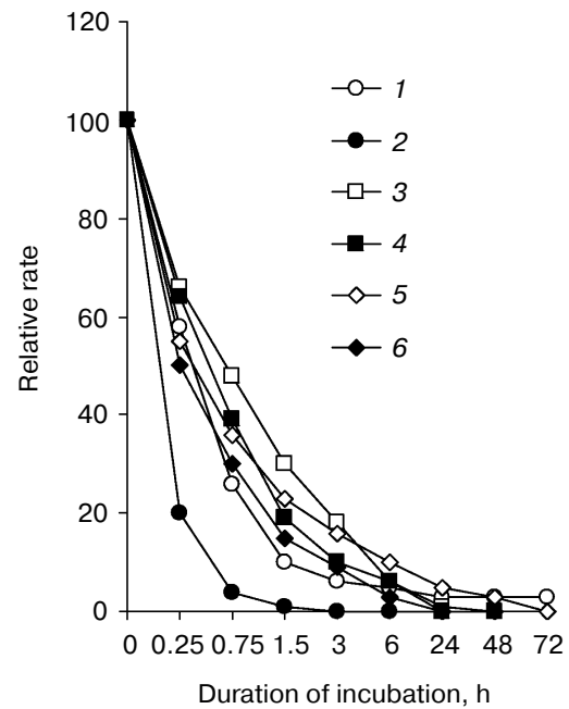
Fig. 2. Effect of duration of incubation at pH 5.5 and 37°C on oxygen uptake and trans-plasma membrane electron transport activities of L. donovani promastigote cells. Cells were incubated at 5% CO 2 + 95% air in MAA/20 medium. Relative rate 100 was considered for DCPIP, ALA, DTNS, NQSA, and K 3 Fe(CN) 6 as well as for oxygen uptake by L. donovani promastigote cells to be 19.32, 1.91, 0.66, 1.11, and 0.42 nmol/min per mg protein and 15.6 nmol O 2 /min per mg protein, respectively. Curves: 1) oxygen uptake; 2) DCPIP reduction; 3) ALA reduction; 4) DTNS reduction; 5) NQSA reduction; 6) ferricyanide reduction. Each point represents the average value of three experiments.
